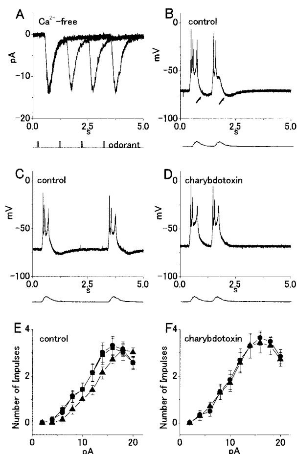
FIGURE 5 Odor adaptation at the level of action potentials. ( A ) Odorant-induced currents with leak current subtracted was recorded from an intact ORC with its cilia attached in a \text{Ca}^{2+} -free bath solution ( V_h = -70 mV). Double pulses of the odorant amyl acetate at the same concentration (100 \mu\text{M} ) and duration (50 ms) were applied to the cell at intervals of 1, 2, and 3 s. Timing of odorant stimulation is indicated by the upward deflection shown below the current traces. ( B and C ) Spiking responses to depolarization induced by injection of the same odorant-induced current traces as in A at intervals of 1 s ( B ) and 3 s ( C ) in control Ringer's solution under current-clamp conditions. Each odorant-induced current trace is shown below the voltage response. ( D ) Spiking responses to depolarization induced by injection of the same current as in ( A , interval = 1 s) in the bath solution containing 100 nM charybdotoxin. ( E ) The relationship between odorant-induced current and spike number of the response to the first (●) and second (▲ and ■) depolarizations in control Ringer's solution. Filled triangles and squares show the intervals of 1 s and 3 s, respectively. Each symbol represents the mean of six cells \pm standard error. ( F ) Relationship between odorant-induced current and spike number of the response to the first (●) and second (▲) depolarizations in the presence of 100 nM charybdotoxin. The interval of the odorant-induced current was 1 s.
