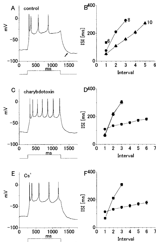
FIGURE 1 Spike frequency accommodation of an isolated ORC. (A, C, and E) Action potentials in response to +8 pA depolarizing current injection in control Ringer's solution (A), 100 nM charybdotoxin (C), or 2 mM CsCl (E). Each voltage response was recorded from the same cell using the \beta -escin perforated patch-clamp technique. (B) Interspike interval (ISI) versus interval number plots were generated in response to 1-s depolarizing current steps of 6 pA (■), 8 pA (●), and 10 pA (▲) in control Ringer's solution. Current intensities are labeled for each plot. Each symbol represents the mean of seven cells \pm standard error. (D) ISI versus interval number plots in response to +8 pA current step in control (■, n = 7 ), 100 nM charybdotoxin (●, n = 7 ), or 2 mM CsCl (▲, n = 4 ). (F) ISI versus interval number plots in response to +8 pA current step in control (■, n = 7 ) or 50 nM iberiotoxin (●, n = 4 ).
